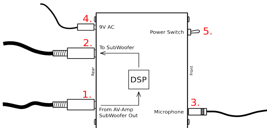
Image 5: Connecter l'ANTI-MODE 8033
